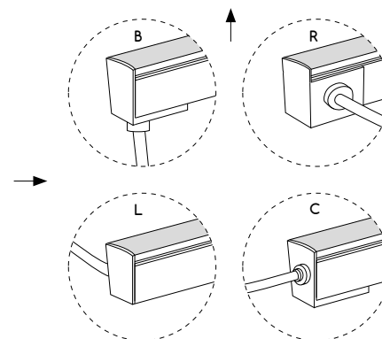
Injected connector options
