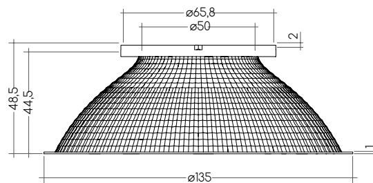
ACD REFLECTOR 150mm 60 D
