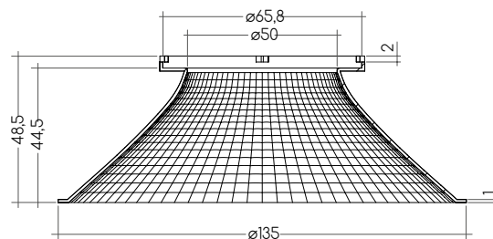
ACD REFLECTOR 150mm 90 D
